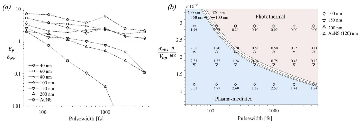
Fig. 5 (a) Calculated ratio of the energy deposited in the plasma ( E_p ) and in the nanoparticle ( E_{NP} ) at the experimental threshold fluencies. (b) Diagram of the ratio \frac{\sigma_{abs} \Lambda}{V_{np} N^2} versus pulse width. The solid black curves correspond to the crossover pulse width t_{p,t} , which marks the transition from plasma-mediated to photothermal cavitation for various nanoparticle sizes (shown in [nm]). The curves were calculated based on eqn (4) and numerical analysis shown in Section S3 of the ESI.† The ratios E_p/E_{NP} for the cases of AuNS, 200 nm, 150 nm, and 100 nm particles, as shown in (a), are included for comparison. For the cases of 80 nm, 60 nm, and 40 nm particles, \frac{\sigma_{abs} \Lambda}{V_{np} N^2} becomes smaller and all their corresponding values reside within the plasma-mediated region, below the transition curve (not shown in the diagram).
