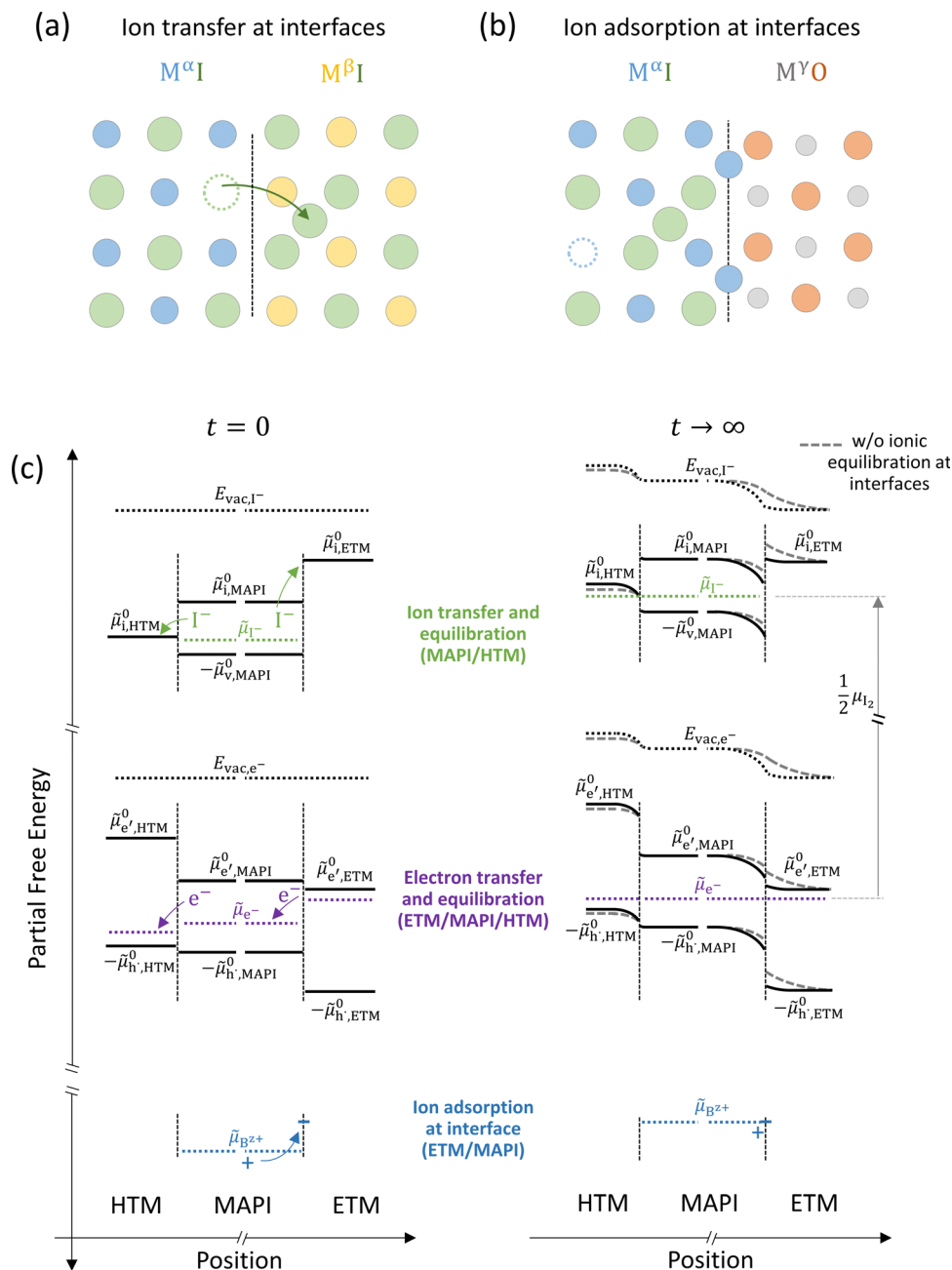
Fig. 7 (a) Ionic equilibration between two metal iodide phases M^\alpha I and M^\beta I , where transfer of I^- from M^\alpha I to M^\beta I increases the concentration of V_{I^-}^\bullet on the left side and of I_i^- on the right side of the interface giving rise to an interfacial equilibrium space charge ( \Delta\mu_i \neq 0 and different standard potentials of defect formations in the two phases are assumed). (b) Metal cation adsorption from a metal iodide M^\alpha I on the interface of a second phase (here an oxide M^\gamma O ) induces a space charge region where positive defects are depleted and the concentration of negative defects (here V_M^\bullet and I_i^- ) is increased. (c) Example of an extended ionic and electronic energy diagram of a MAPI solar cell in the dark at equilibrium where the interfaces are highlighted. Ion transfer (here I^- ) and ion adsorption (here B^{z+} adsorbed at the MAPI/ETM interface, e.g. Pb^{2+} adsorbed on TiO_2 surface 47 ) can have significant repercussion on the chemical and electrostatic situation at interfaces. The situations upon contact ( t = 0 ) and after equilibration ( t \rightarrow \infty ) are shown. In the right diagram, dashed lines indicate the situation where ionic equilibration with contact materials is not considered.
