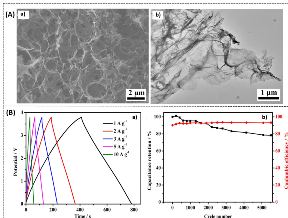
Fig. 13 (A) SEM images of (a) UPGA and (b) TEM image of UPGA, (B) electrochemical Response of UPGA: (a) GCD response (b) cycling stability vs. coulombic efficiency at 1 \text{A g}^{-1} . Reprinted with permission, 93 Copyright (2021) from Elsevier.
