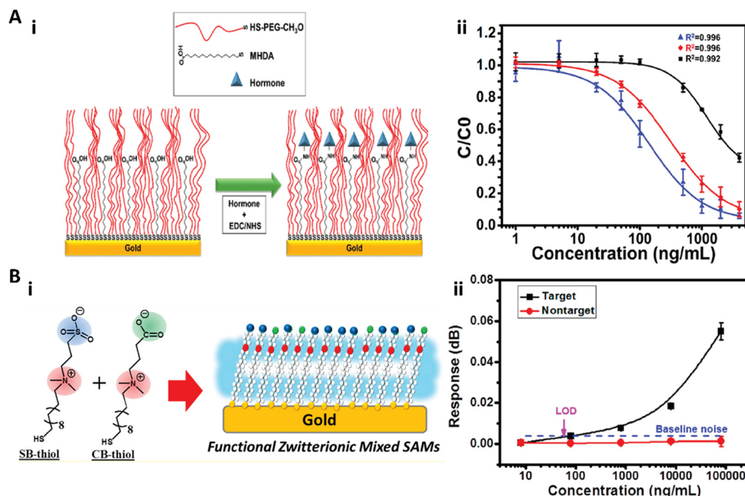
Fig. 2 A-i) The schematic illustration of the mixed SAM formed on the Au film. The thiolated poly(ethylene glycol) ( \text{CH}_3\text{O}-\text{PEG}-\text{SH} ) in the mixed SAM served as the spacer and the antifouling agent to prevent the nonspecific adsorption, while the 16-mercaptohexadecanoic acid (MHDA) was used for hormone immobilization. A-ii) Multiplex hormone calibration curves of the SPR sensor for insulin (blue), glucagon (red), and somatostatin (black). Reproduced from ref. 56, Copyright 2018 American Chemical Society. B-i) The schematic illustration of the functional zwitterionic mixed SAMs with sulfobetaine-thiol (SB-thiol) and carboxybetaine-thiol (CB-thiol). B-ii) Calibration curve for detection of the target and nontarget secondary antibodies with the SPR biosensor. Reproduced from ref. 61, Copyright 2019 American Chemical Society.
