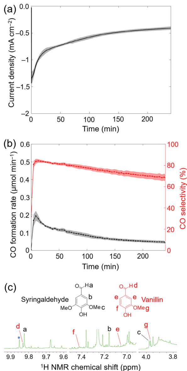
Fig. 4 Electrolysis of 20 vol% \text{CO}_2 gas flow with CP|CoP L at the cathode coupled to lignin conversion at the anode with CP|MWCNT. (a) Current density as a function of time. (b) CO formation rate and selectivity during electrolysis at the cathode. (c) ^1\text{H} NMR spectrum recorded in \text{CDCl}_3 of the anolyte containing lignin after 4 h electrocatalysis showing the emergence of aldehydes and methoxy groups. Experiments were performed in triplicates, and the standard deviation are represented as shaded area (a, b). Reaction conditions: (a and b) Electrolysis (two electrode configuration) at U_{\text{app}} = -3 V. Anolyte: 0.1 M \text{Na}_2\text{CO}_3 , lignin fraction obtained from pre-treating 250 mg lignocellulose in 1:1 MeCN:H 2 O; anode: CP|MWCNT. Catholyte: 0.1 M \text{NaHCO}_3 in H 2 O with a flow of 20 vol% \text{CO}_2 (balanced with \text{N}_2 ) 9 mL min -1 ; cathode: CP|CoP L ; bipolar membrane; room temperature. (c) The asterisk (*) highlights the additional aldehyde signal formed from lignin electrooxidation.
