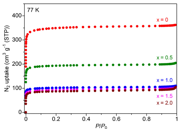
Fig. 2 \text{N}_2 adsorption isotherms of \text{UiO-66} \cap \{\text{Mg}(\text{TFSI})_2\}_x ( x = 0-2.0 ) at 77 K.
