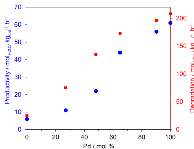
Fig. 1 The effect of Pd: Au ratio on the catalytic activity of 0.66% PdAu/TS-1 catalysts towards the direct synthesis (●) and subsequent degradation (■) of \text{H}_2\text{O}_2 . \text{H}_2\text{O}_2 direct synthesis reaction conditions: catalyst (0.01 g), \text{H}_2\text{O} (2.9 g), MeOH (5.6 g), 5% \text{H}_2/\text{CO}_2 (420 psi), 25% \text{O}_2/\text{CO}_2 (160 psi), 0.5 h, 2 °C, 1200 rpm. \text{H}_2\text{O}_2 degradation reaction conditions: catalyst (0.01 g), \text{H}_2\text{O}_2 (50 wt% 0.68 g), \text{H}_2\text{O} (2.22 g), MeOH (5.6 g), 5% \text{H}_2/\text{CO}_2 (420 psi), 0.5 h, 2 °C, 1200 rpm.
