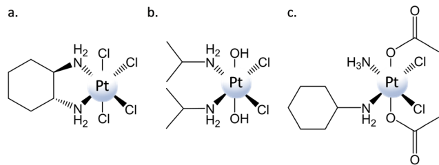
Scheme 1 Structure of (a) tetraplatin, (b) iproplatin, and (c) satraplatin/JM216.
