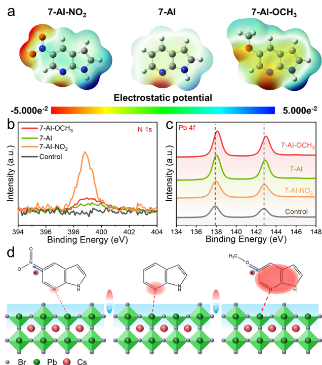
Fig. 1 (a) Molecular structures and electrostatic potential maps of 5-nitro-7-azaindole (7-AI- \text{NO}_2 ), 7-azaindole (7-AI), and 5-methoxy-7-azaindole (7-AI- \text{OCH}_3 ). XPS spectra of (b) N 1s and (c) Pb 4f in \text{CsPbBr}_3 films without and with organic molecule treatment. (d) Schematic diagram of electron-transfer-induced coulomb force regulation and the N atom passivated uncoordinated \text{Pb}^{2+} .
