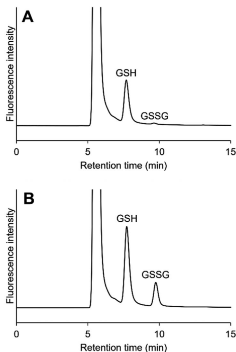
Fig. 3 Typical chromatograms of GSH and GSSG in PC12 cell samples. (A) Unspiked, (B) spiked with 40 μM GSH and 10 μM GSSG.
