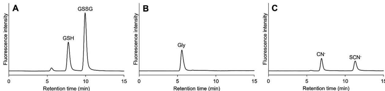
Fig. 2 Typical chromatograms of reduced and oxidized glutathiones (GSH and GSSG), glycine (Gly), and cyanide and thiocyanate (CN − , and SCN − ). (A) 5 μM GSH and 5 μM GSSG, (B) 0.1 μM Gly, (C) 0.1 μM CN − and 0.1 μM SCN − . Column: Scherzo SM-C18 (3 μm, 150 × 4.6 mm i.d.). Mobile phase: 75 mM acetate buffer (pH 5.0).
