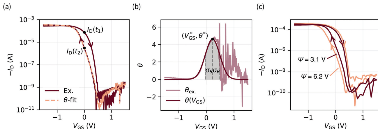
Fig. 3 (a) Transfer characteristic with labeled points of the on \rightarrow off ( I_D(t_1) ) and off \rightarrow on ( I_D(t_2) ) curve ( V_{DS} = -0.1 V). The orange curve was obtained through eqn (3) with fitting parameters for \theta(V_{GS}) (eqn (2)) of V_{GS}^* = 0.22 V, \theta^* = 4.62 , and \sigma_\theta = 0.26 V. (b) Experimental data of eqn (1) ( \theta_{ex.} ) are approximated by a Gaussian-type expression \theta(V_{GS}) (eqn (2)). (c) \psi is defined as the integral of \theta(V_{GS}) in boundaries of the scan range (eqn (4)). Two transfer curves are shown with assigned \psi parameters for comparison. A linear plot of this data is provided in Fig. S8 (ESI†).
