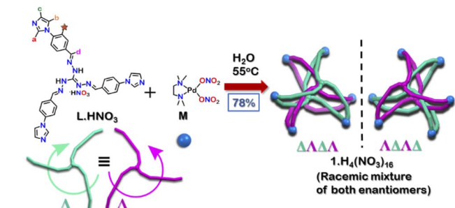
Scheme 1 Synthesis of interlocked Pd 6 cage 1 using a triimidazole donor L \cdot HNO_3 .
