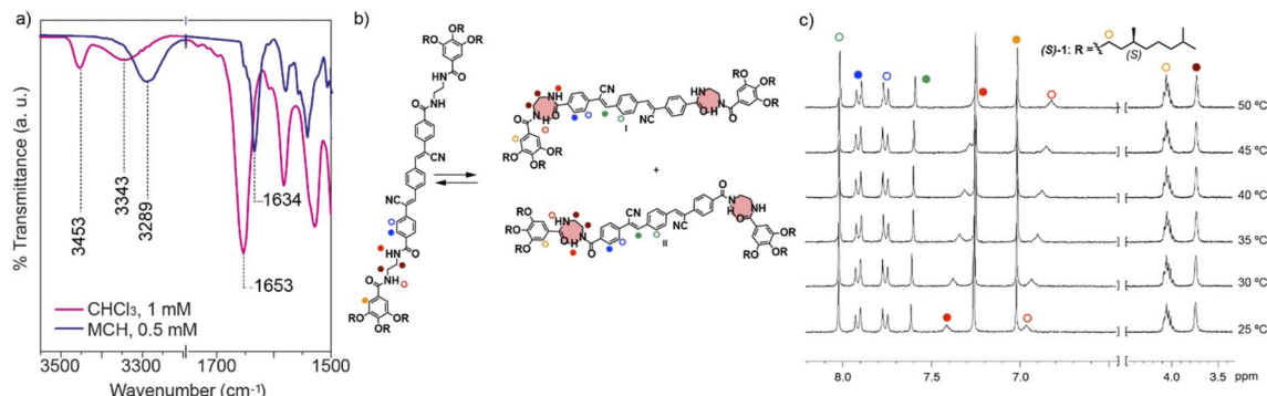
Fig. 2 (a) Partial FTIR spectra of (R)-1 in CHCl 3 and MCH; (b) schematic illustration of the equilibrium between the two monomeric species, the totally unbound and the intramolecularly H-bonded, of cyano-luminogens 1; (c) partial 1 H-NMR spectra of (S)-1 at different temperatures (300 MHz, CDCl 3 , c T = 1 mM).
