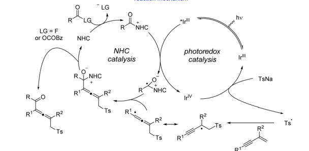
Scheme 19 NHC/Ir co-catalyzed three-component 1,4-sulfonylacylation of 1,3-enynes.
