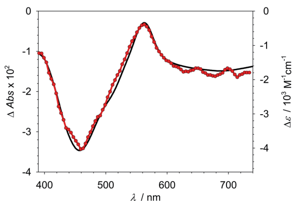
Fig. 3 Absorption changes 50 ns after laser flash excitation (650 nm) of [\text{Fe(II)}(\text{btz})_3](\text{PF}_6)_2 2 in MeCN : MeOH (4 : 3) with C 8 F 17 I (0.45 M) (●) and difference spectrum between [\text{Fe(II)}(\text{btz})_3](\text{PF}_6)_2 2 and [\text{Fe(III)}(\text{btz})_3](\text{PF}_6)_3 1 ( 1 – 2 , –).
