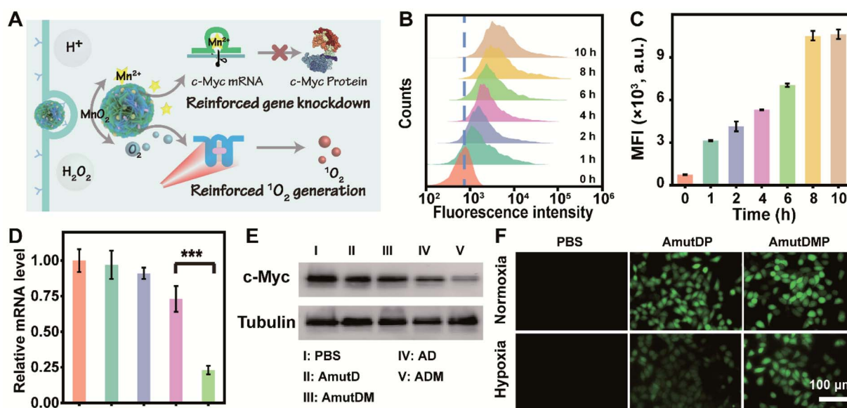
Fig. 2 DNAzyme-mediated enhanced gene silencing and 1 O 2 generation in cancer cells by the active targeting and responsive DNA nano-assembly. (A) Depiction of cancer-targeted, stimulus-triggered, and self-reinforced gene knockdown and 1 O 2 generation in live cells. (B and C) Time-dependent internalization of Cy5-labeled AMDP into 4T1 cells determined by flow cytometry. Representative histogram results (B) and quantification of the mean fluorescence intensity (MFI) (C) are shown. (D) qRT-PCR analysis of c-Myc mRNA in 4T1 cells incubated separately with PBS (I), AmutD (II), AmutDM (III), AD (IV), and ADM (V). Results are presented as means ± standard deviation (SD) ( n = 3). Statistical significance was calculated by one-way ANOVA with Tukey's post hoc test: *** p < 0.001. (E) Western blot analysis of c-Myc protein expression of 4T1 cells with different treatments. (F) Detection of 1 O 2 generation in 4T1 cells by DCFH-DA. The cells were incubated with PBS, AmutDP, and AmutDMP in both normoxia and hypoxia under 660 nm laser irradiation (0.2 W cm -2 ) for 5 min. AmutD, the DNA nanostructure with the aptamer and mutant DNAzyme; AmutDM, the DNA nanostructure with the aptamer, mutant DNAzyme, and MnO 2 ; AmutDMP, the DNA nanostructure with the aptamer, mutant DNAzyme, MnO 2 , and photosensitizer.
