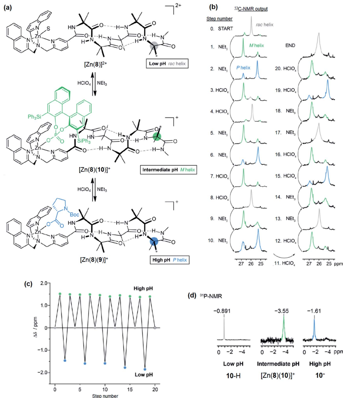
Fig. 11 (a) pH-induced exchange of 9^- and 10^- with [Zn(8)]^+ , (b) ^{13}\text{C} -NMR output from the terminal ^{13}\text{C} -labelled Aib reporter group, (c) difference in chemical shift between major and minor peaks ( \delta_{\text{major}} - \delta_{\text{minor}} ) after addition, (d) ^{31}\text{P} NMR spectrum of the system at low, intermediate and high pH.
