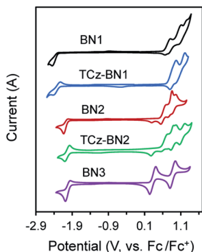
Fig. 4 Cyclic voltammograms (CV) for all compounds. The CV curves were measured at room temperature with 0.1 M solution of [n\text{-Bu}_4\text{N}]\text{PF}_6 in dichloromethane for the oxidation and reduction scan (vs. \text{Fc}/\text{Fc}^+ ).
