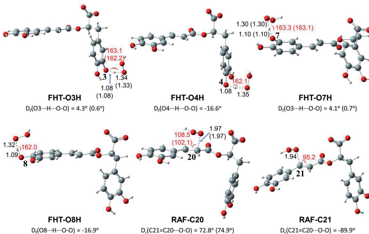
Fig. 3 Optimized structures of the transition states (TSs) for FHT and RAF reactions of rosmarinate mono-anion ( \text{RA}^- ) towards \text{HOO}\cdot radicals in water calculated at the M05-2X/6-311++G(2df,2p) level of theory. D_f is the OHOO dihedral angle of the FHT TSs; D_r is the CCOO one of the RAF TSs. The values in parentheses correspond to the geometrical parameters obtained in the PEA phase.
