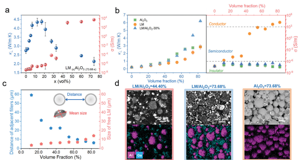
Fig. 2 Thermally conductive yet electrically insulating properties of the PUPDM composite. (a) Thermal conductivity and electrical conductivity of the PUPDM/LM/Al 2 O 3 composite as a function of the LM/Al 2 O 3 volume ratio. Note that the total volume content of the binary filler is 73.68%. (b) Out-of-plane thermal and electrical conductivity as a function of the volume fraction of the binary filler for different PUPDM composites. Note that the LM/Al 2 O 3 volume ratio is 30%. (c) Average distance between adjacent fillers and an average size of the free LM as a function of the volume fraction of the binary filler in the PUPDM/LM/Al 2 O 3 composite. (d) Scanning electron microscopy images and the elemental mapping images of the PUPDM/LM/Al 2 O 3 and PUPDM/Al 2 O 3 composites.
