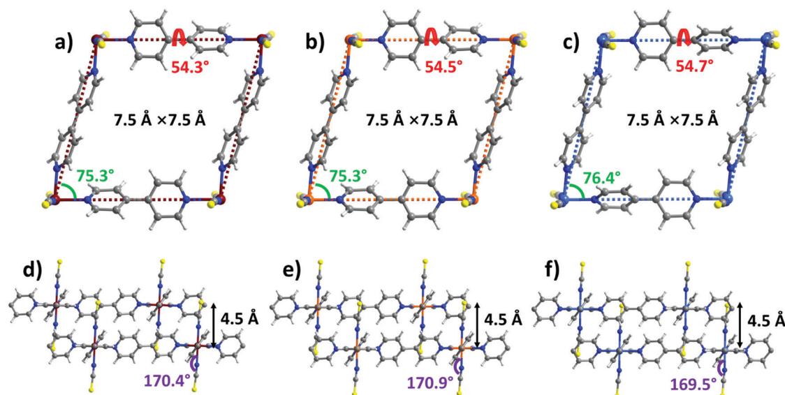
Fig. 1 Comparison of the crystal structures of sql-1-M-NCS . (a and d) M = \text{Fe} ; (b and e) M = \text{Co} ; (c and f) M = \text{Ni} .
