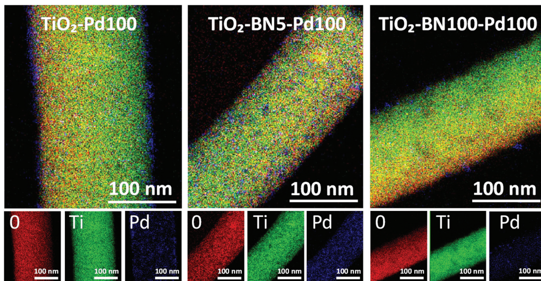
Fig. 5 EDS elemental mapping of TiO 2 -Pd100, TiO 2 -BN5-Pd100 and TiO 2 -BN100-Pd100 nanofibers.
