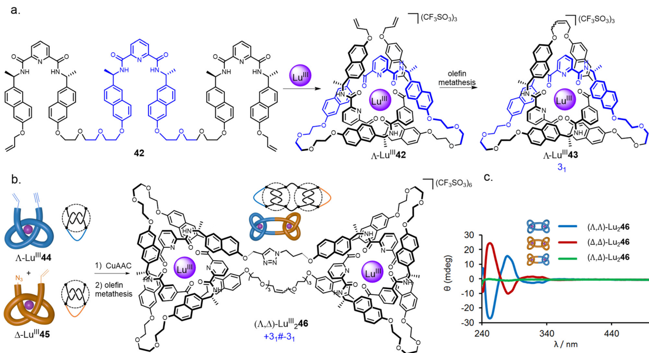
Fig. 15 (a) Synthesis of trefoil knot \Delta\text{-Lu}^{\text{III}}\mathbf{43} by folding a single ligand around a lanthanide ion. 80 (b) Stereoselective synthesis of composite knots with tangle representations, here represented by square knot synthesis. 82 (c) CD spectra of granny and square knots \text{Lu}_2\mathbf{46} . 82 Reproduced from ref. 82 through a CC-BY license.
