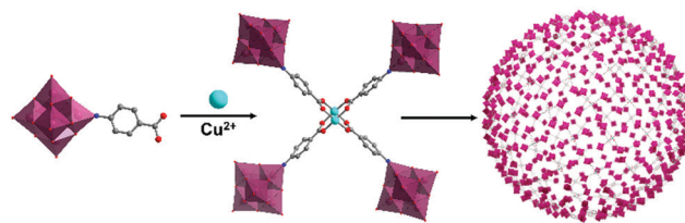
Fig. 8 Model of the electrostatically assembled "blackberry" structure formed by the self-assembly of tetrameric hexamolybdate hybrids. This figure has been adapted from ref. 92 with permission from the American Chemical Society, copyright 2013.
