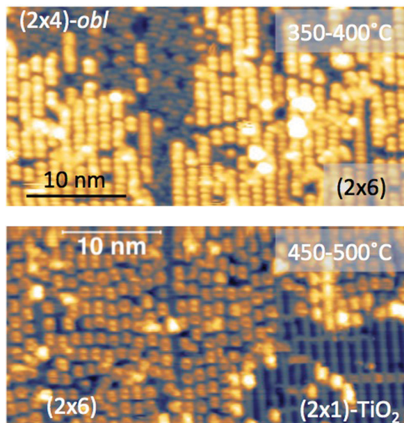
Fig. 16 Top: STM image (Colibri tip) showing the coexistence of (2 \times 4) -obl and (2 \times 6) -rect phases, as obtained by thermal desorption at 350\text{--}400\text{ }^{\circ}\text{C} of a bi-layer film grown at RT (+2.5 V, 60 pA); molecules in the new phase display two symmetric lobes, much brighter than those in the (2 \times 4) -obl phase. Bottom: The same film after annealing to 450\text{--}500\text{ }^{\circ}\text{C} , as imaged close to a (2 \times 1) reconstructed region, which shows a significant dewetting (+1.5 V, 80 pA).
