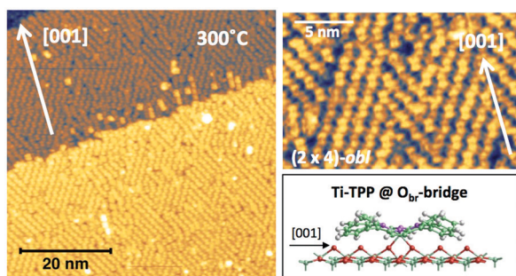
Fig. 13 Left: Large scale image of 1 ML obtained upon thermal desorption at 300 °C of a bi-layer of 2H-TPP deposited at RT (+2.5V, 100 pA); all terraces are covered with an extended (2 × 4)-obl phase, entirely composed of metalated TPP molecules. Right: A smaller scale image of the same film puts in evidence the saddle-shape of the metalated molecules, and a small asymmetry with respect to the major axis due to the small azimuthal rotation of the molecules in the ordered phase, as compared to the isolated ones. Inset panel: A side-view of the equilibrium configuration of an isolated TiO 2 br -TPP molecules puts in evidence the bonding of molecular Ti with the two O br atoms underneath.
