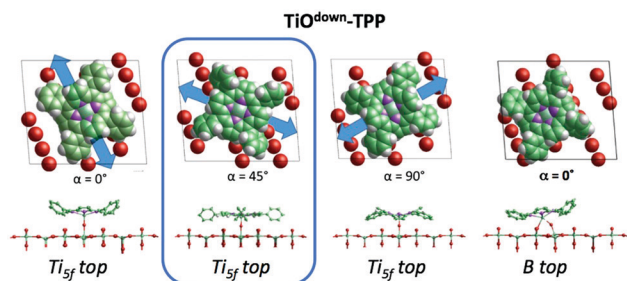
Fig. 22 Side and top views of the equilibrium configurations for different azimuthal orientations of \text{TiO}^{\text{down-TPP}} adsorbed atop a \text{Ti}_{5f} atom, as well as above the B adatom site, after coordination to an adjacent \text{O}_{\text{br}} atom.
