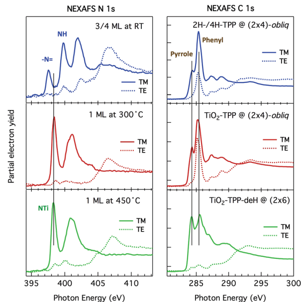
Fig. 17 NEXAFS spectra measured in partial electron yield at the N and C K-edges, left and right panels, respectively, at RT, 300\text{ }^{\circ}\text{C} and 450\text{ }^{\circ}\text{C} , corresponding to different molecular species and symmetry phases; spectra measured in TM and TE polarization are represented as full and dotted lines, respectively. The surface was azimuthally oriented to keep the scattering plane along the [001] direction. In this geometry, the TE spectra are measured with the electric field transverse to the rows, where the molecules display a slightly larger intensity of \pi -symmetry resonances than along the rows, hence yielding the maximum tilt angle/molecular distortion in any chemical state. Adapted from ref. 49 with permission from the Royal Society of Chemistry, Copyright 2017.
