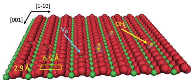
Fig. 1 Perspective view of the \text{TiO}_2(110) surface termination where oxygen and titanium atoms are represented by red and green spheres, respectively. Point defects, such as oxygen vacancies ( \text{V}_\text{O} ) and hydroxyls ( \text{OH}_\text{b} ), are also indicated.
