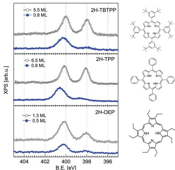
Fig. 3 Comparison between the monolayer (filled blue markers) and multilayer (open black markers) photoemission spectra of the N 1s peak for three different porphyrins. All films were grown on the substrate at room temperature (RT). Adapted from ref. 45 with permission from the PCCP Owner Societies, Copyright 2015.
