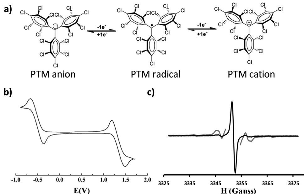
Fig. 1 (a) Molecular structure of the PTM radical and its corresponding oxidation and reduction to the cation and anion, respectively. (b) Representative cyclic voltammogram of a PTM radical in CH_2Cl_2 , with 0.1 M n-Bu_4NPF_6 (vs. Ag/AgCl ). Adapted from ref. 4 Copyright 2012 Royal Society of Chemistry. (c) EPR spectrum of a PTM radical recorded at room temperature in deoxygenated CH_2Cl_2 ( g = 2.0023 ). In grey the same spectrum recorded with a higher power to better appreciate the ^{13}C hyperfine coupling.
