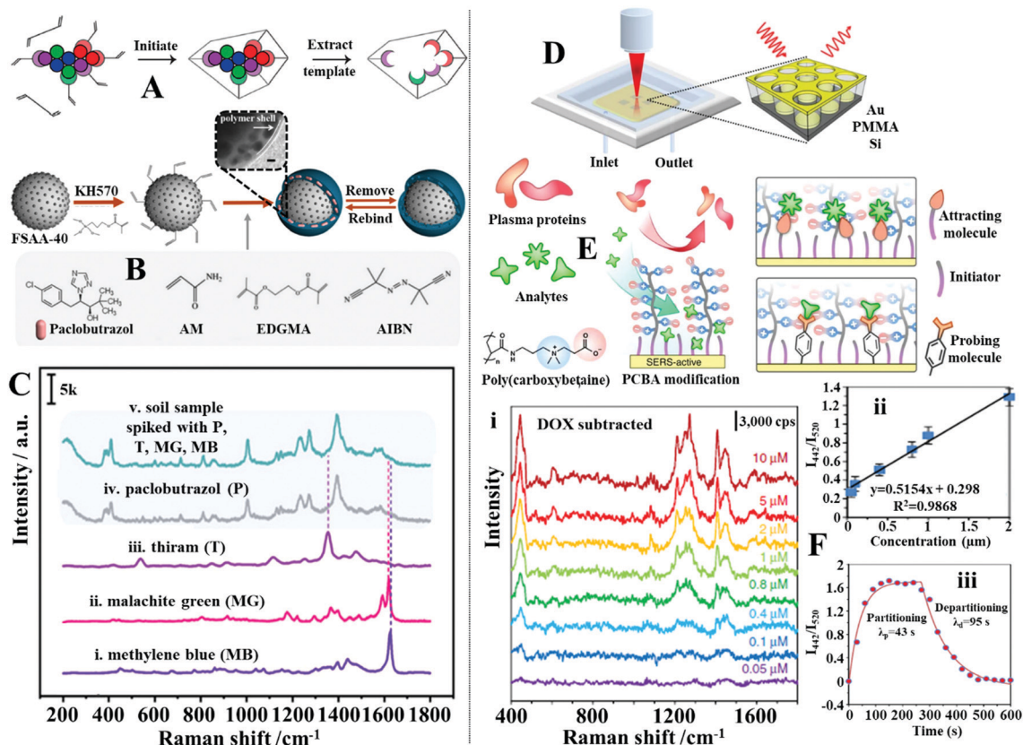
Fig. 12 (A) Schematic illustrations of the working principles of molecular imprinted polymers (MIPs); (B) schematic illustration of the preparation of \text{Fe}_3\text{O}_4@SiO_2-Au@Ag (FSAA) MIPs. Inset shows a TEM image of the product FSAA MIPs; (C) SERS spectra set demonstrating the selectivity of the FSAA MIP sensors. Spectra (i–iv) correspond to the SERS signals of the target analyte paclobutrazol and three contaminants, namely, thiram, malachite green and methylene blue. Spectrum v corresponds to the SERS signals obtained from a soil sample spiked with all four chemicals; (D) schematic illustrations of the SERS optofluidic system; (E) schematic illustrations of the different types of mixed self-assembled monolayers functionalized on the surface of the enhancing material to achieve anti-fouling and target recognition; (F) panel (i) show SERS spectra of Doxorubicin in plasma ultrafiltrate control at concentrations ranging from 0.05 to 10 \mu\text{M} . The background signals from plasma have been subtracted. Panel (ii) shows the linear region of the Doxorubicin detection curve generated by plotting the average intensity ratio of the doxorubicin peak at 442 \text{cm}^{-1} and plasma peak at 520 \text{cm}^{-1} as a function of doxorubicin concentration. The error bars stand for standard deviations obtained from three replicates. Panel (iii) shows partitioning and departitioning kinetics of 20 mM Doxorubicin in plasma on the anti-fouling SERS sensor. Panel (A) reproduced with permission from ref. 178, copyright 2017 American Chemical Society. Panel (B and C) adapted with permission from ref. 75, copyright 2020 American Chemical Society. Panel (D–F) adapted with permission from ref. 182, copyright Springer Nature Limited.
