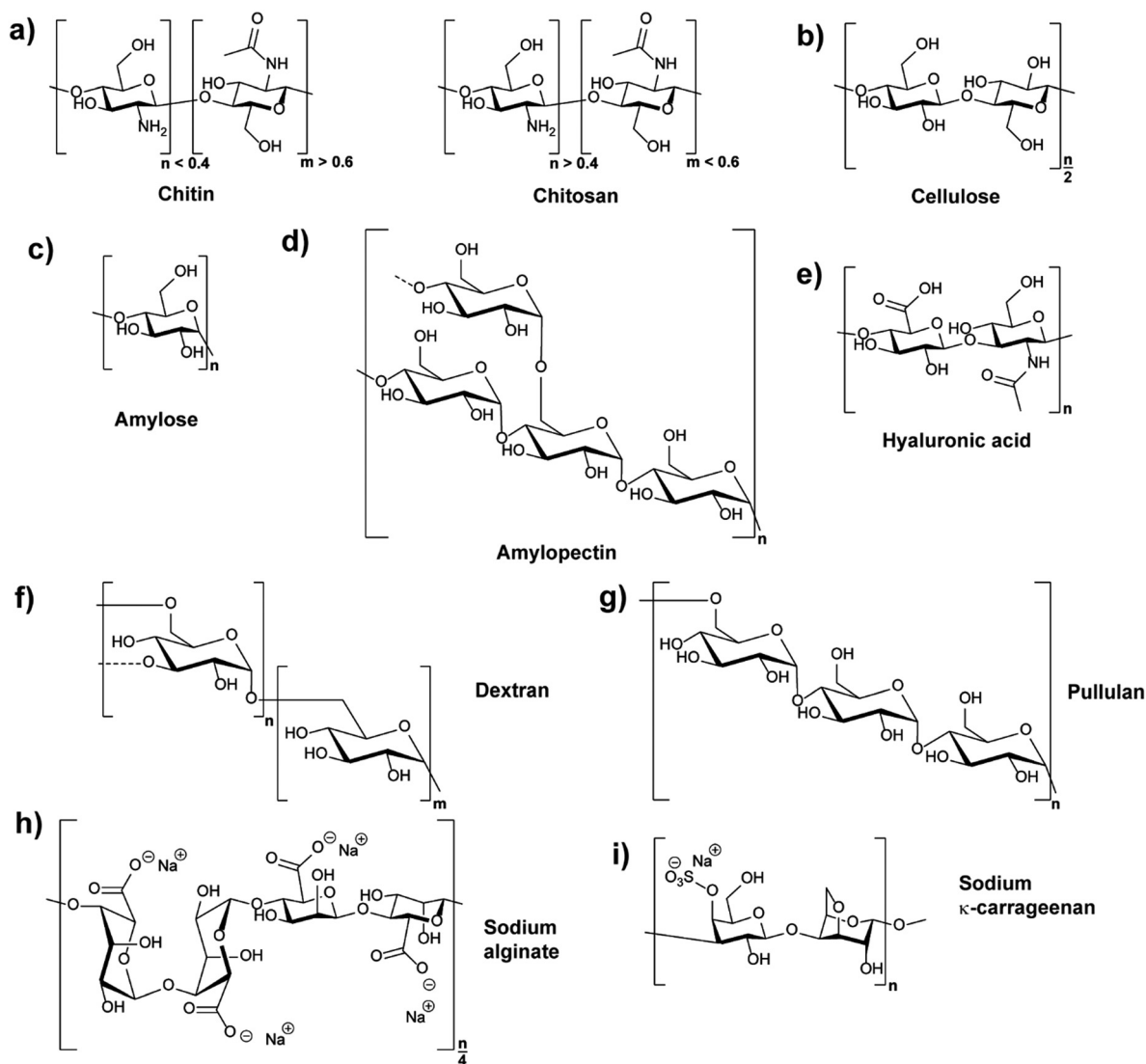
Fig. 1 Chemical structures of polysaccharides: (a) chitin (CH) and its derivative from N -deacetylation chitosan (CS), (b) cellulose (CL), (c) and (d) structures of two different polymers coexisting in starch, amylose and amylopectin (dashed lines indicate branches), (e) hyaluronic acid (HA), (f) dextran (DEX) (dashed lines indicate branches), (g) pullulan (PL), (h) sodium alginate ( \alpha -L-guluronic acid- \alpha -L-guluronic acid- \beta -D-mannuronic acid- \beta -D-mannuronic acid sequence shown), and (i) \kappa -carrageenan ( \kappa -CRG).
