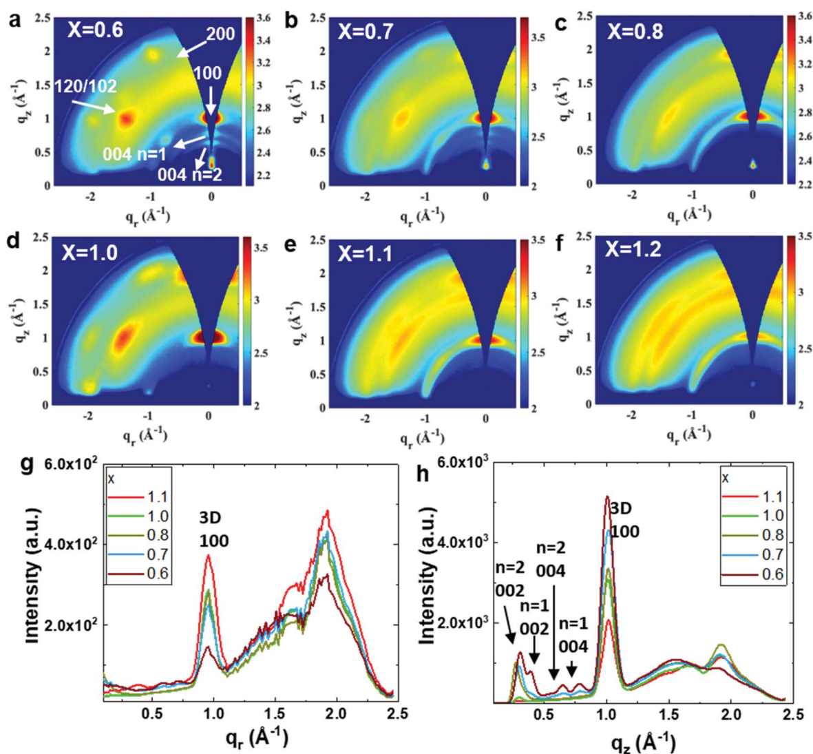
Fig. 2 GIWAXS patterns of (a) the \text{PEA}_{0.08}\text{FA}_{0.6}\text{SnI}_3 , (b) \text{PEA}_{0.08}\text{FA}_{0.7}\text{SnI}_3 , (c) \text{PEA}_{0.08}\text{FA}_{0.8}\text{SnI}_3 , (d) \text{PEA}_{0.08}\text{FA}_{1.0}\text{SnI}_3 , (e) \text{PEA}_{0.08}\text{FA}_{1.1}\text{SnI}_3 and (f) \text{PEA}_{0.08}\text{FA}_{1.2}\text{SnI}_3 films. The images were recorded using an incident angle of 2^\circ . Line-cut data of the \text{PEA}_{0.08}\text{FA}_x\text{SnI}_3 ( x = 0.6 – 1.1 ) films along (g) q_r and (h) q_z directions.
