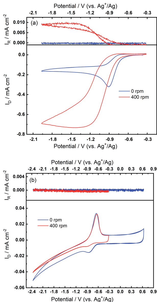
Fig. 7 RRDE measurements at 100 mV s^{-1} with rotation speeds of 0 rpm and 400 rpm (a) before and (b) after the oxidation peak appears in O_2 -bubbled 0.1 M TBAClO_4 /0.01 M Ca(ClO_4)_2 /DMSO. The disc and ring electrodes are GC and Pt, respectively, and the potential of ring is -0.37 V. A potential limit of -2.37 V is set in (b), in accordance with previous CVs wherein the reversible OER peak can be found.
