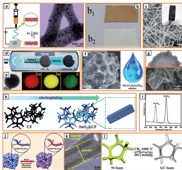
Fig. 8 Electrospinning, spray drying, electrodeposition, and CVD. (a) Electrospinning process and the corresponding microstructure of \text{Sb}@\text{CN} nanofibers. Reproduced with permission. 2 Copyright 2020, Elsevier. (b) As-spun preasphaltene/PAN (b1) and PAN (b2) fibers. Reproduced with permission. 27 Copyright 2020, American Chemical Society. (c) SEM images of \text{CuO}/\text{Cu} -NCNFs. Reproduced with permission. 46 Copyright 2020, Elsevier. (d) Schematic illustration of the spraying process and (e) corresponding elemental mapping of the \text{CoTe}_2 -C composite. Reproduced with permission. 64 Copyright 2020, Elsevier. (f) SEM of the obtained N-doped interconnected carbon spheres and the \text{NaCl}/\text{C}_6\text{H}_{17}\text{N}_3\text{O}_7 precursor for spraying. Reproduced with permission. 81 Copyright 2019, The Royal Society of Chemistry. (g) Morphology of the activated crumpled graphene after the spray drying process. Reproduced with permission. 99 Copyright 2020, Wiley. (h) Schematic of the electrodeposition process of \text{SnO}_2@\text{CF} and (i) XRD spectrum after deposition. Reproduced with permission. 16 Copyright 2020, The Royal Society of Chemistry. (j) CVD for the fabrication of red \text{P}@\text{AC} . Reproduced with permission. 119 Copyright 2020, Elsevier. (k) Microstructure of multiwalled hierarchical carbon nanotube after CVD. Reproduced with permission. 125 Copyright 2018, Wiley. (l) CVD for the synthesis of graphitic carbon foam. Reproduced with permission. 129 Copyright 2019, The Royal Society of Chemistry.
