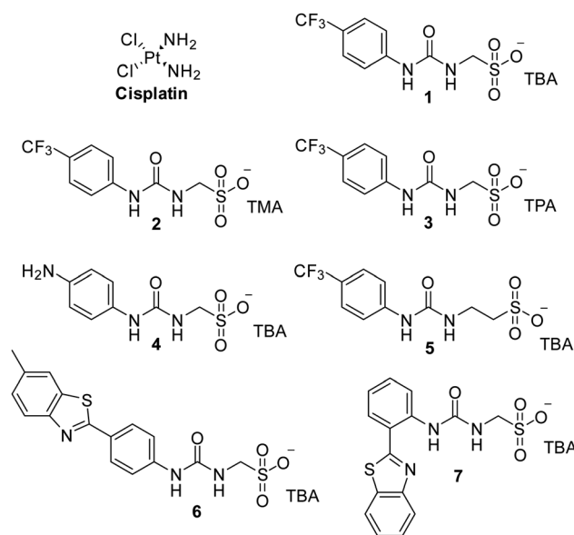
Fig. 1 Chemical structure of cisplatin and SSAs 1–7. TBA = tetrabutylammonium, TMA = tetramethylammonium, TPA = tripropylammonium.
