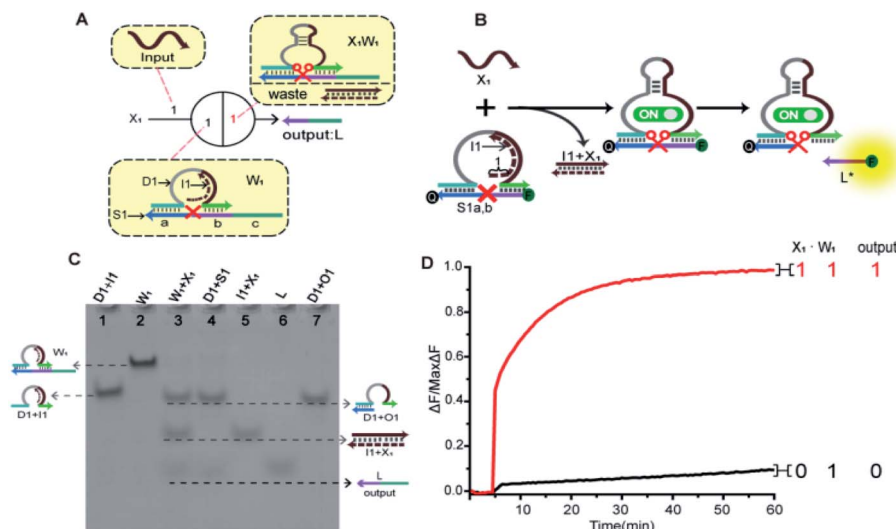
Fig. 2 (A) Abstract diagram of the weight unit 1 motif and its DNA implementation. The black numbers indicate the initial relative concentration. Red number indicates relative product concentrations, and different colours indicate distinct DNA sequences. S1a is the left (3'-end) recognition domain of substrate strand 1 ( S1 ), while S1b is the right (5'-end) recognition domain of S1 . (B) Illustration of the weight unit 1. The substrate strand sequence is S1a,b , 5'-end fluorophore FAM and 3'-end quencher BHQ1 for fluorescent signal determination. (C) Native PAGE analysis of the weight unit 1. The strands and complex involved were labelled above the lane number. Lane 1, complex ( D1 + I1 ) consists of DNAzyme 1 ( D1 ) and inhibitor 1 ( I1 ); lane 2, weight unit 1 ( W_1 ) consists of D1 , I1 and S1 ; lane 3, products of W_1 triggered by input X_1 ; lane 4, products of D1 digestion; lane 5, complex ( I1 + X_1 ); lane 6, output strand L ; lane 7, complex ( D1 + O1 ). (D) Time-dependent fluorescence changes according to different inputs. The standard concentration was 1 \times = 0.2 \mu\text{M} , [X_1] and [W_1] was 1 : 1. The red curve reflects the reaction with the addition of X_1 and the black curve is the case with no input.
