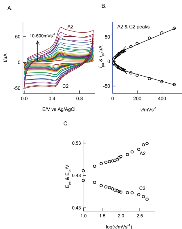
Fig. 2 (A) CV response of effect of scan rate (10–500 mV \text{s}^{-1} ) on GCE/Nf–MWCNT@ \text{PhOCH}_3 -Redox in pH2 KCl–HCl buffer. Plots of (B) anodic peak current ( i_{\text{pa}} ) and cathodic peak current ( i_{\text{pc}} ) vs. scan rate and E_{\text{pa}} and E_{\text{pc}} vs. log of scan rate (C) for A2/C2 peak.
