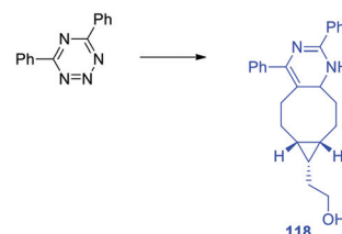
Scheme 26 Reaction of 2,6-diphenyl-1,3,4,5-tetrazine with cyclooctyne.
