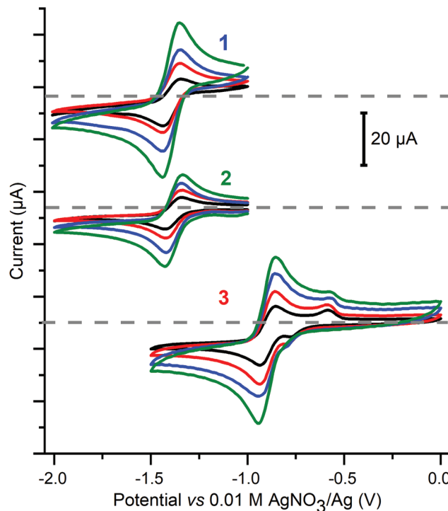
Fig. 7 Cyclic voltammetry of the reversible redox processes seen at negative potentials for 1 mM MeCN solutions of 1 (top, E_{1/2} = -1.39 V, \Delta E = 0.09 V, D = 7.7 \times 10^{-6} cm ^2 s ^{-1} ), 2 (middle, E_{1/2} = -1.39 V, \Delta E = 0.09 V, D = 3.4 \times 10^{-6} cm ^2 s ^{-1} ), and 3 (bottom, E_{1/2} = -0.89 V, \Delta E = 0.09 V, D = 5.4 \times 10^{-6} cm ^2 s ^{-1} ). Conditions: 0.1 M (Bu _4 N)PF _6 , glassy carbon working electrode ( d = 3 mm, A = 0.071 cm ^2 ), 293 K, vs. 0.01 M AgNO _3 /Ag. In this system E_{1/2}(\text{Fc}^+/\text{Fc}) = 0.09 \pm 0.01 V, with \Delta E = 0.09 V, and this was unchanged even after 6 h of electrolysis (Fig. S31†). Scan direction: for 1 and 2 -1.0 \rightarrow -2.0 \rightarrow -1.0 V, for 3 0.0 \rightarrow -1.5 \rightarrow 0.0 V; scan rate: 50 (black), 100 (red), 200 (blue) and 400 (green) mV s ^{-1} ; grey dashed lines correspond to zero current for each set of CVs.
