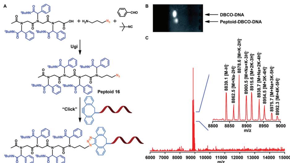
Fig. 8 (A) Conjugation of sequence-controlled peptoid 16 to DNA (DNA : peptoid molar ratio = 1, 24 h reaction in \text{CH}_3\text{CN}/\text{PBS} ). (B) Gel electrophoresis result for the peptoid–DNA conjugation reaction. (C) MALDI-TOF-MS analysis of DNA conjugates.
