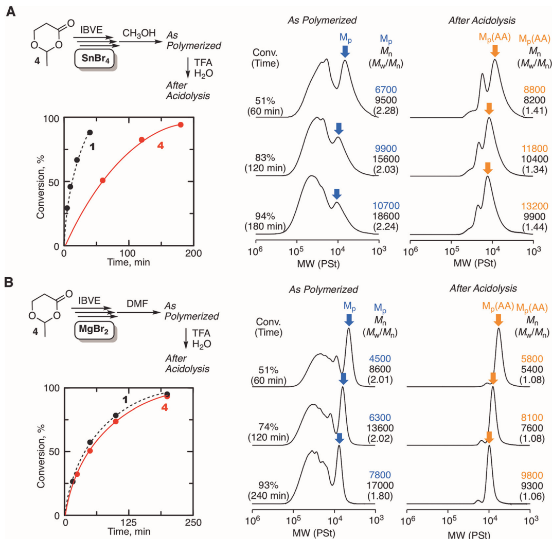
Fig. 5 Comparison between \text{SnBr}_4 (A) and \text{MgBr}_2 (B) as a catalyst for the ring-expansion cationic polymerization of IBVE with 4 : [\text{IBVE}]_0/[\text{4}]_0/[\text{SnBr}_4] or [\text{MgBr}_2]_0/[\text{DTBMP}]_0 = 380/5.0/5.0 or 10/0.15 mM in toluene (for \text{SnBr}_4 ) or toluene/ \text{Et}_2\text{O} (90/10 vol%) (for \text{MgBr}_2 ) at 0^\circ\text{C} .
