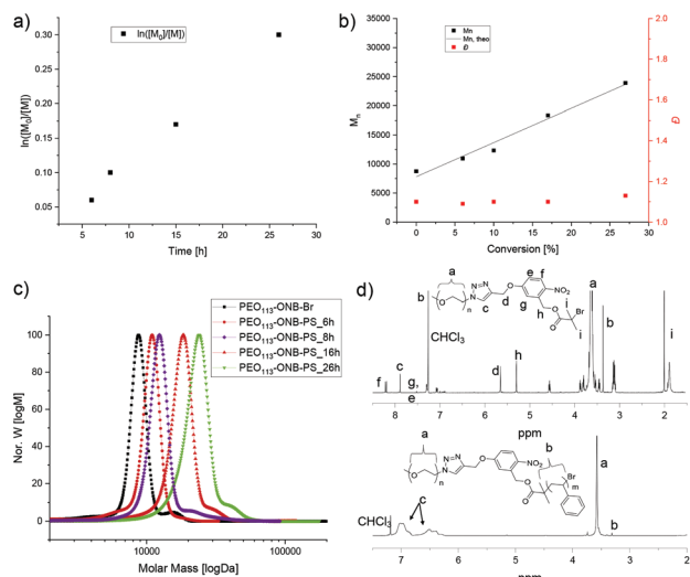
Fig. 1 Synthesis and characterization of PEO-ONB- b -PS diblock copolymers. (a) Logarithmic plot of monomer consumption versus time. (b) Linear relation of molecular weight and polymer dispersity versus conversion. (c) GPC traces during the polymerization of PEO 113 -ONB- b -PS at varying t . (d) 1 H NMR of PEO 113 -ONB-Br and PEO 113 -ONB- b -PS 90 .
