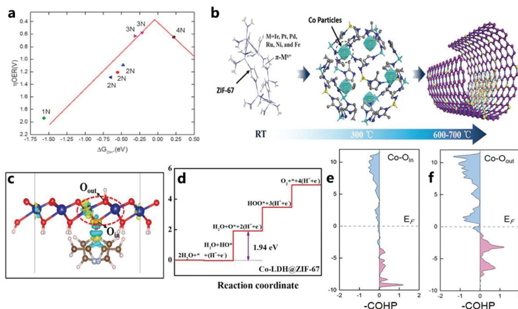
Fig. 23 (a) ZIF-67-xN (x = 1–4) volcano diagram related to the OER catalytic activity and OH adsorption energy on the Co site. 138 Copyright © 2017 Elsevier Ltd. All rights reserved. (b) Illustration of locations of metal cations and \pi electrons. (At room temperature, metal cations are initially related to \pi electrons. At 300 °C, the metal atoms embedded in cobalt form single atoms. At 600–700 °C, cobalt forms on the base carbon atom.) 137 Copyright © 2019 Wiley-VCH Verlag GmbH & Co. KGaA, Weinheim. (c) The charge density difference of the underlying layer for Co-LDH@ZIF-67, and (d) the Gibbs free energy step diagram of the OER on Co-LDH@ZIF-67. pCOHP for (e) Co–O in and (f) Co–O out in Co-LDH@ZIF-67. 187 Copyright © 2020 The Authors. Published by Wiley-VCH GmbH.
