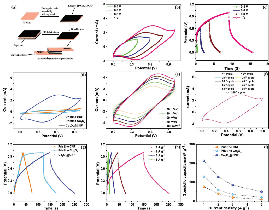
Fig. 6 Electrochemical performance of the SSC on the pristine \text{Co}_3\text{O}_4 nanoparticles, pristine CNF and 1\text{D Co}_3\text{O}_4@\text{CNF} hybrid electrodes: (a) simple schematic illustration of the SSC device that consisted of similar two 1\text{D Co}_3\text{O}_4@\text{CNF} hybrid electrodes, (b and c) CV and GCD curves collected at various voltage windows, (d) comparison CV curve at 20\text{ mV s}^{-1} , (e) CV curve at, (f) cycling CV curves over 100 cycles, (g and h) comparison GCD curve at 1\text{ A g}^{-1} and at various current densities, respectively, (i) specific capacitance at different current densities.
