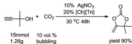
Fig. 2 A gram-scale reaction under low concentration of \text{CO}_2 using \text{AgNO}_3 as the catalyst and [Ch][Tri] as the cocatalyst.
