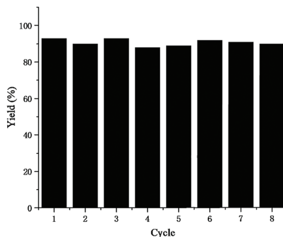
Fig. 3 Recycling experiments using \text{AgNO}_3 as the catalyst and [Ch][Tri] as the cocatalyst.
