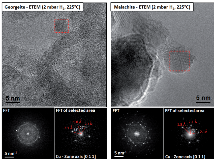
Fig. 1 The microstructures of the reduced georgeite and malachite precursors characterized by ETEM in 2 mbar \text{H}_2 at 225 °C. Both samples reveal distinct Cu nanoparticles distributed on ZnO as confirmed by FFT analysis. The reduced malachite sample reveals in general larger Cu nanoparticles compared to the georgeite sample. Reproduced with permission from ref. 7.
