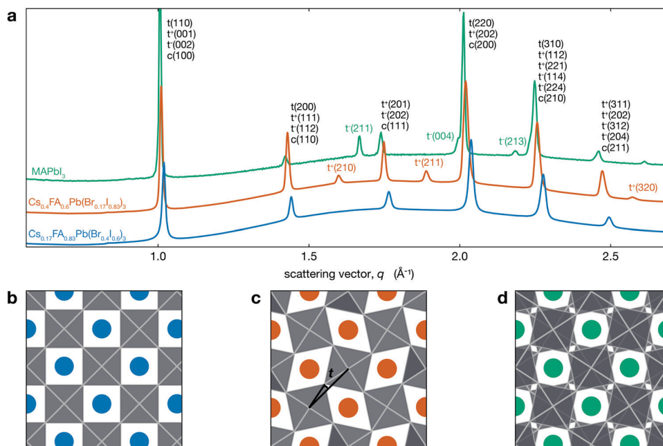
Fig. 1 (a) XRD patterns for different Cs y FA 1- y Pb(Br x I 1- x ) 3 compositions exhibiting both tetragonal a^0a^0c^+ (tetragonal peaks indexed with t^+ ) and cubic a^0a^0a^0 structures as well as the a^0a^0c^- (tetragonal peaks indexed with t^- ) phase of MAPbI 3 (MAPbI 3 data from Schelhas et al. 50 ). The y -axis is linear in intensity (arbitrary units not shown) with an offset between the three patterns. Views of (b) a^0a^0a^0 , (c) a^0a^0c^+ , and (d) a^0a^0c^- structures looking down the c -axis. Blue, orange and green spheres represent the A-site cation, and the PBX 6 octahedra are shown in grey. The tilt angle t we consider here is the angle between the black lines in (c).
