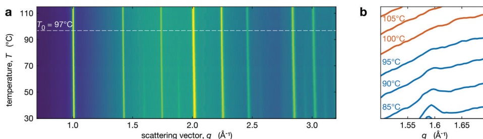
Fig. 2 (a) Temperature XRD map for Cs 0.4 FA 0.6 Pb(Br 0.17 I 0.83 ) 3 with the extracted T_0 (temperature where film is purely cubic) indicated by a dashed line. (b) Evolution of the integrated intensity of the t(210) superlattice peak. Temperature is increasing moving up in the vertical direction. The y -axis is linear and represents the intensity counts in arbitrary units.
