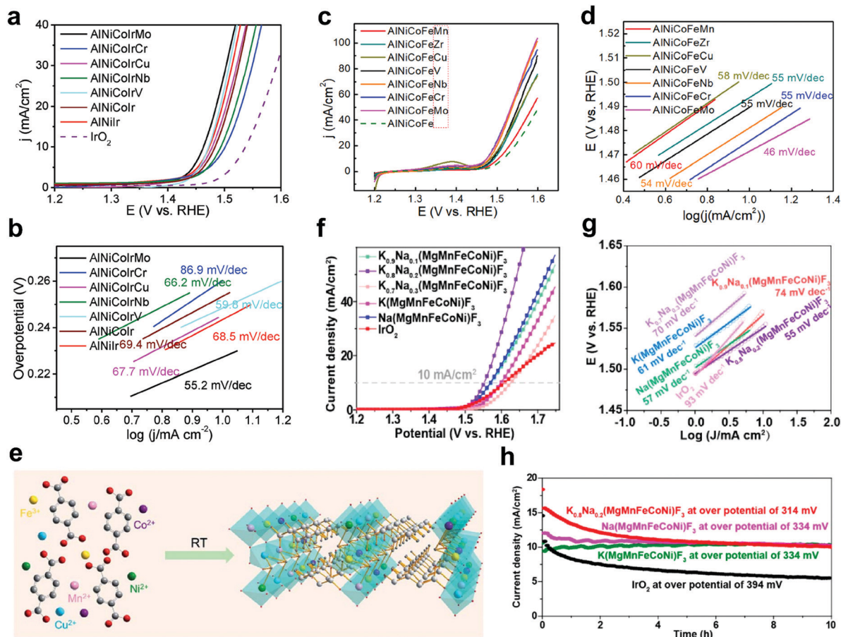
Fig. 6 (a) Linear sweep voltammetry and (b) the corresponding Tafel curves of different AlCoNi-based HEAs and IrO 2 in 0.5 M H 2 SO 4 solution. Reproduced with permission. 39 Copyright 2019, Wiley-VCH. (c) Linear sweep voltammetry and (d) the corresponding Tafel curves for different AlCoNiFe-based HEAs in 1 M KOH solution. Reproduced with permission. 41 Copyright 2019, American Chemical Society. (e) Synthetic procedure for the preparation of MnFeCoNiCu-based HE-MOF at ambient conditions. Reproduced with permission. 42 Copyright 2019, The Royal Society of Chemistry. (f) Linear sweep voltammetry and (g) the corresponding Tafel curves as well as (h) chronoamperometric recording of IrO 2 and Na x K 1-x (FeCoNiMnMg)F 3 in 1 M KOH solution. Reproduced with permission. 43 Copyright 2020, American Chemical Society.
