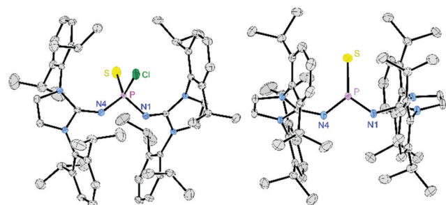
Fig. 1 Solid-state structure of 3 (left) and [4][BARF_{24}] (right). Hydrogen atoms, solvent molecules and the anion of [4][BARF_{24}] are omitted for clarity. Ellipsoids are drawn at 50% probability. Only one of the two crystallographically independent molecules of 3 and only one part of the disordered isopropyl group and N_2PSCl moiety is depicted. Selected bond lengths [Å] and angles ^\circ of [4][BARF_{24}] : P–N1 1.5578(12), P–N4 1.5606(12), P–S 1.8967(5), N1–P–N4 108.02(6), N1–P–S 124.79(5), N4–P–S 127.17(5).
