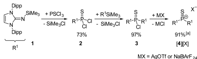
Scheme 2 Synthesis of [4][OTf] and [4][BARF_{24}] . Dipp = 2,6-diisopropylphenyl, OTf^- = trifluoromethanesulfonate, BARF_{24}^- = tetrakis[3,5-bis(trifluoromethyl)phenyl]borate. a yield for MX = NaBARF 24 .
