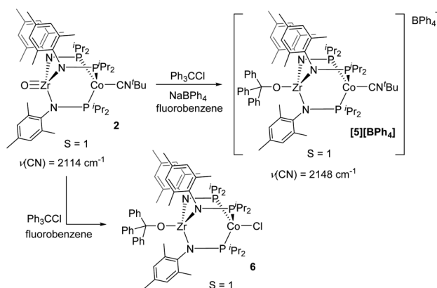
Scheme 2 The reactivity of 2 with \text{Ph}_3\text{C}^+ reagents.
