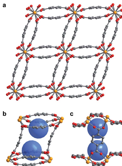
Fig. 1 (a) Single crystal X-ray diffraction structure of 1-H 2 O viewed along the c -axis, showing the parallelepipedal pores. (b) Truncated structure showing one of the pores of 1-H 2 O along the crystallographic c -axis, with the two identical binding pockets of the pore depicted as blue spheres. (c) The same view as in (b), rotated by 90° to visualize the bowl-shaped arrangement of three bdc 2- linkers that form the cap of each binding pocket. Orange, red, and grey spheres represent U, O, and C atoms, respectively; solvent and H atoms are omitted for clarity.
