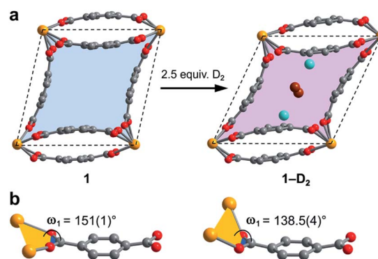
Fig. 5 (a) Illustration of pores in 1 and 1-D 2 (dosed with 2.5 equiv. \text{D}_2 per pore). The pore contraction upon \text{D}_2 dosing is highlighted by the colored blue and purple areas within the crystallographic ab -plane. Tilting of the pores to facilitate contraction is illustrated by idealized parallelograms (dashed lines) with corners defined by uranium atoms. Adsorbed \text{D}_2 molecules inside the pores of 1-D 2 are represented as aquamarine spheres for adsorption site I and as brown spheres for adsorption site II. Each \text{D}_2 super atom at site II is shared between two neighboring pores, accordingly the two depicted site II super atoms together account for an occupancy of one \text{D}_2 molecule per pore. (b) Comparison of the dihedral angles \omega_1 as described in the text ( \omega_2 is not shown, but is the corresponding angle at the other end of the linker), representing the main structural distortion undergone by 1 upon adsorption of \text{D}_2 . Orange, red, and grey spheres represent U, O, and C atoms, respectively.
