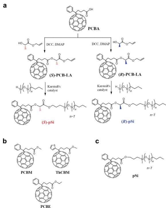
Fig. 1 (a) Synthetic routes for (S)-pSi and (R)-pSi. Chemical structures of (b) the achiral fullerene derivatives used for the inside of the films, PCBM, ThCBM, and PCBE, and (c) pSi.
