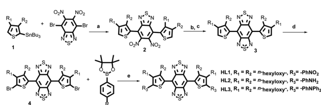
Fig. 2 The synthetic routes of HL1–HL3 . Reagents and conditions: (a) Pd(PPh 3 ) 4 and THF; (b) Zn, NH 4 Cl, and CH 2 Cl 2 /MeOH/H 2 O; (c) PhNSO 2 , TMSCl, and pyridine, two steps; (d) NBS, HBr, and DMF/CH 3 CN; (e) PdCl 2 (dppf) 2 CH 2 Cl 2 and K 2 CO 3 .
